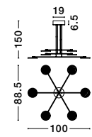
SCOPE . 9695254 Triac Dimmable Black Metal & Acrylic LED 51 Watt 230 Volt 6376Lm 3000K IP20 D: 100 W: 88.5 H: 150 cm
