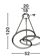
MENTON - 9147113 Triac Dimmable Sandy Coffee Aluminium & Acrylic LED 43 Watt 230 Volt 3013Lm 3000K IP20 D: 52 H1: 50 H2: 120 cm
