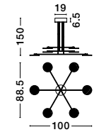
SCOPE - 9695255 Triac Dimmable Black & Gold Metal & Acrylic LED 51 Watt 230 Volt 6376Lm 3000K IP20 D: 100 W: 88.5 H: 150 cm
