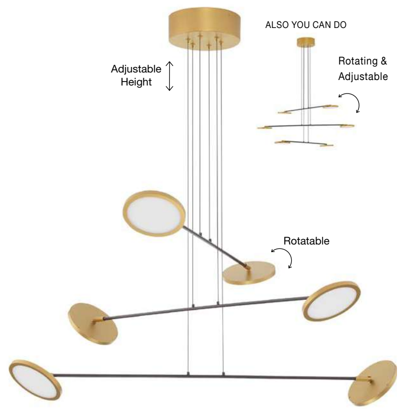
SCOPE - 9695255 Triac Dimmable Black & Gold Metal & Acrylic LED 51 Watt 230 Volt 6376Lm 3000K IP20 D: 100 W: 88.5 H: 150 cm
