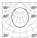
CRI≥90 12W 110° 1200lm 3000K
