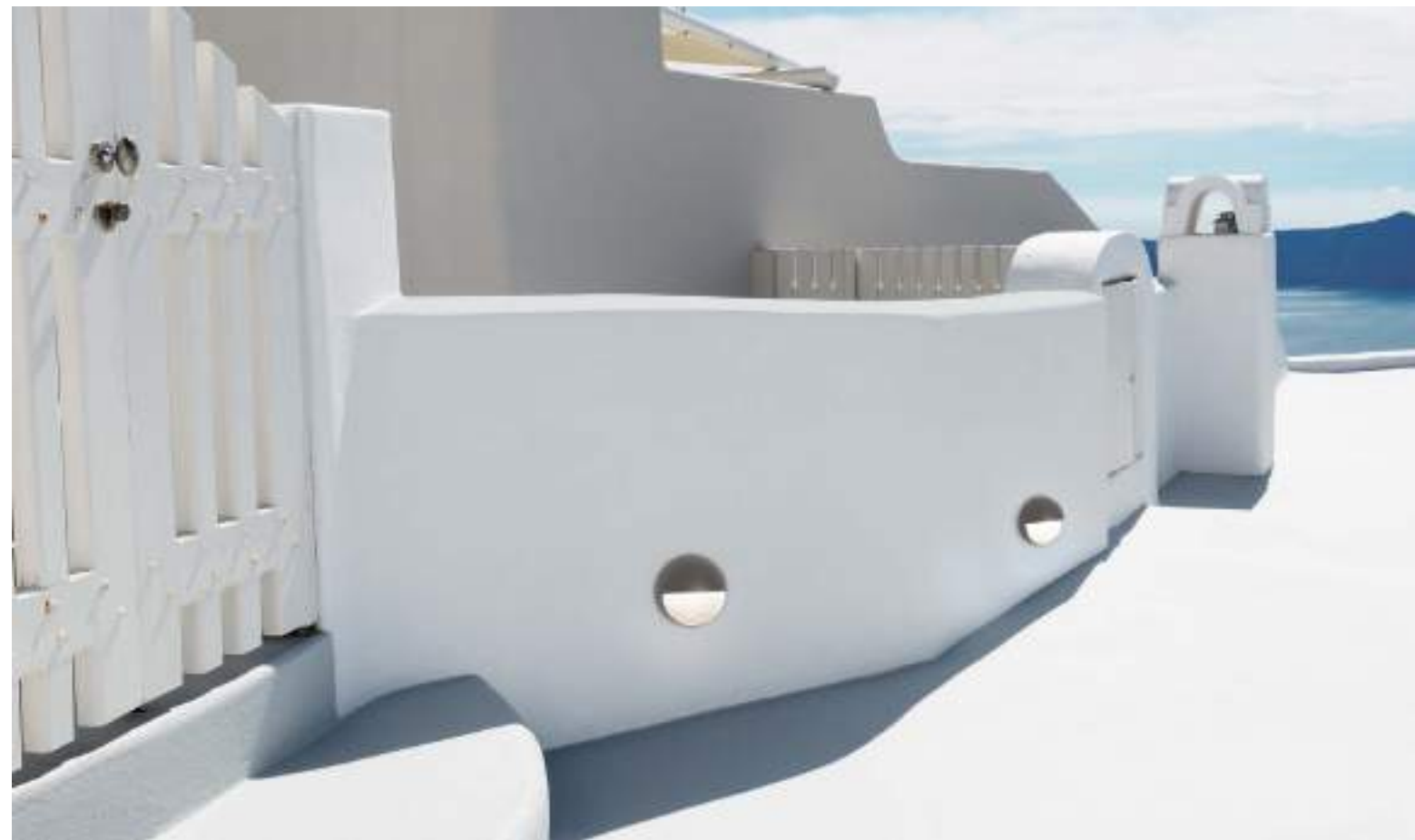
LUTON - 8403624 Dark Gray ABS LED 1.2 Watt 90Lm 3000K IP65 100-220 Volt 50Hz RC Driver Included L: 12.5 W: 3.3 H: 12.5 cm
