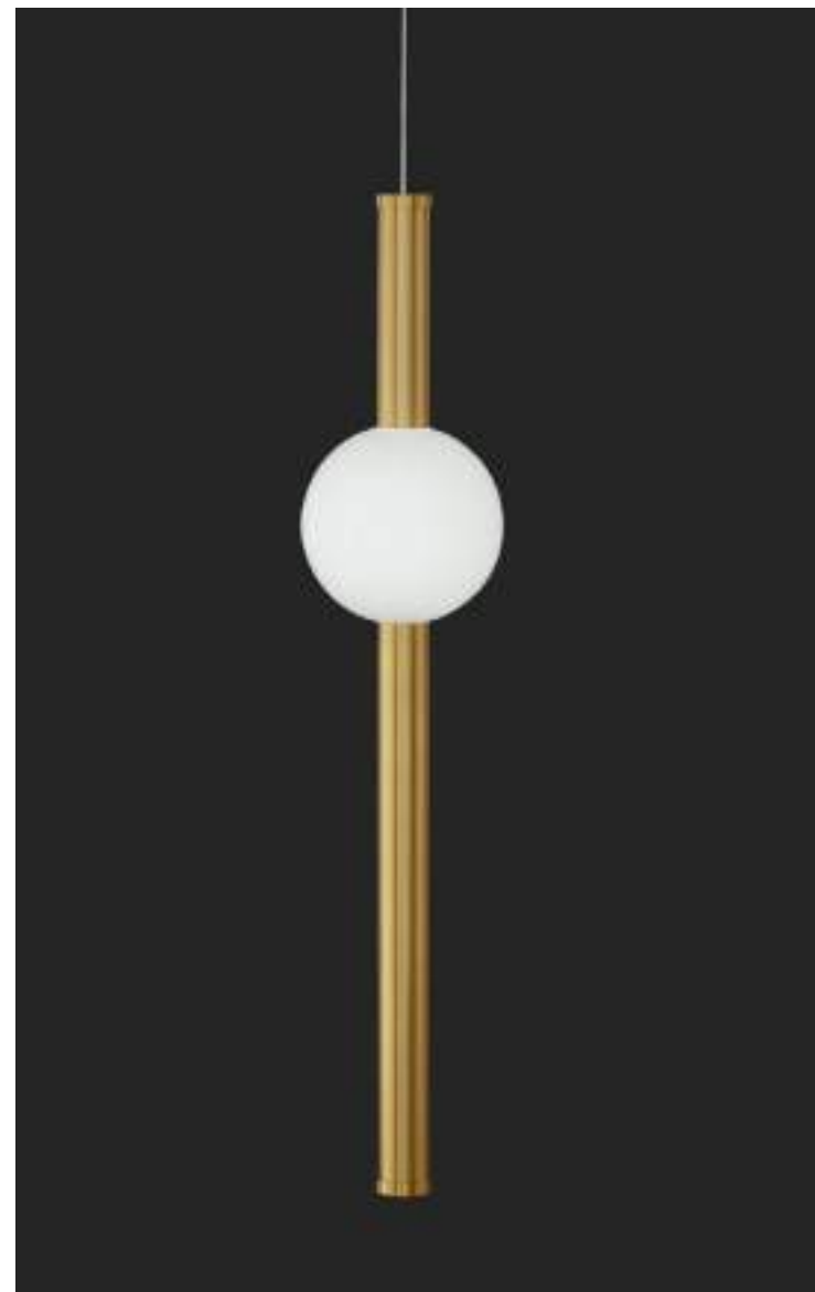
Neutron
