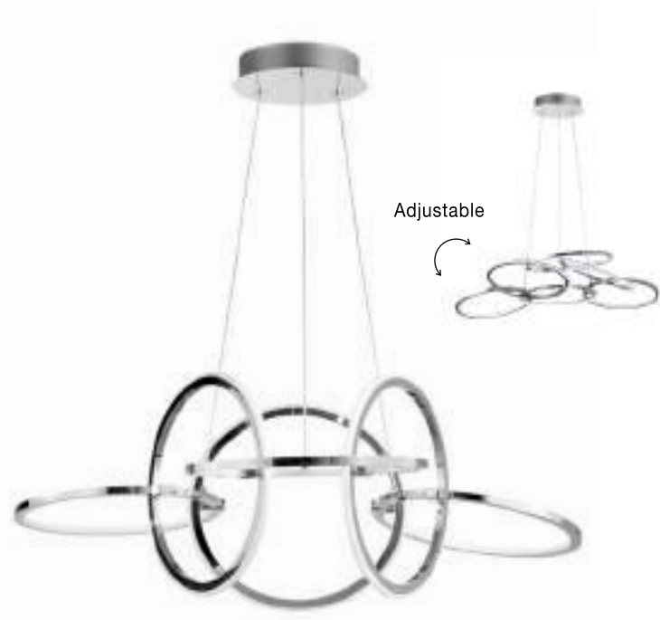
DANTE - 9008012 Chrome Aluminium & Acrylic Adjustable LED 50 Watt 230 Volt 3000Lm 3000K IP20 D: 75 H: 150 cm
