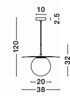
OBBIT - 9988381 Opal Glass Gold Metal LED E27 1x12 Watt 230 Volt IP20 Bulb Excluded D: 20 H: 32 H 2 : 120 cm
